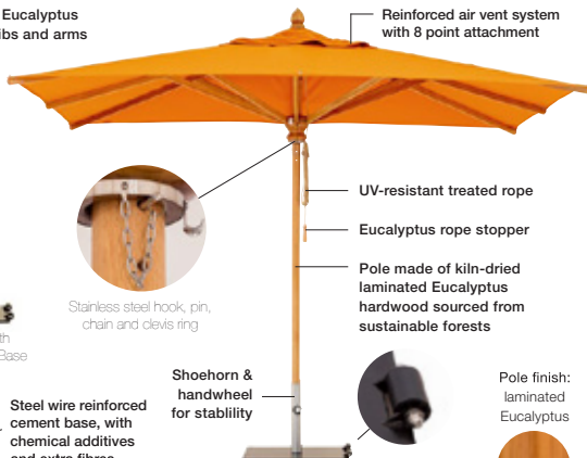
Rectangular model on Square Metal Plate Base with rollers for mobility
